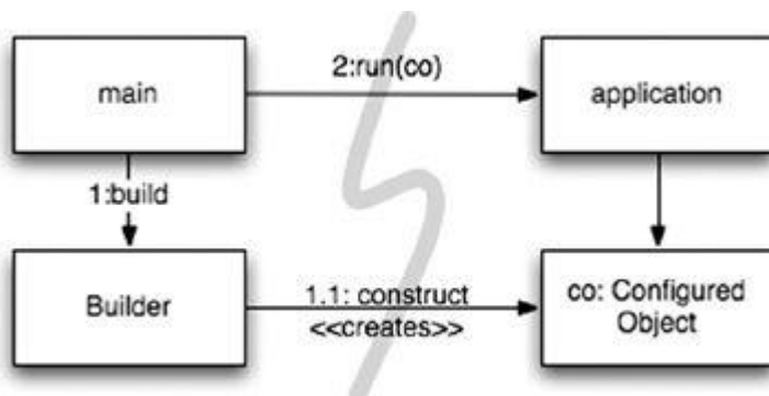
Figure 11-1 Separating construction in main()
