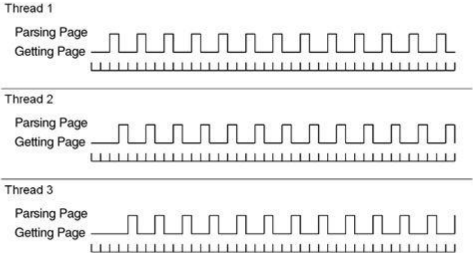
Figure A-2 Three concurrent threads
